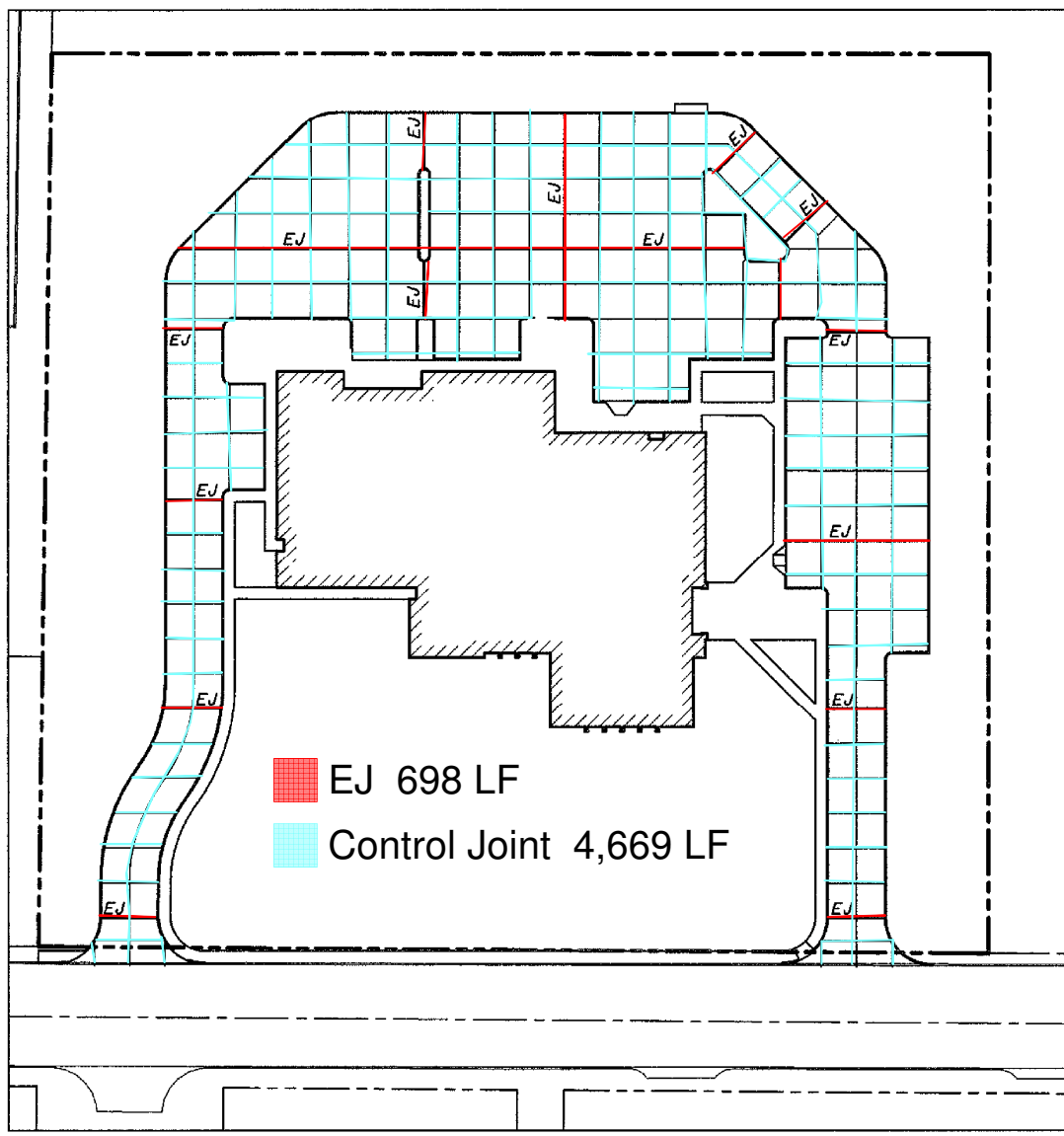
SUGGESTED JOINTING PLAN SCALE 1" = 50'
